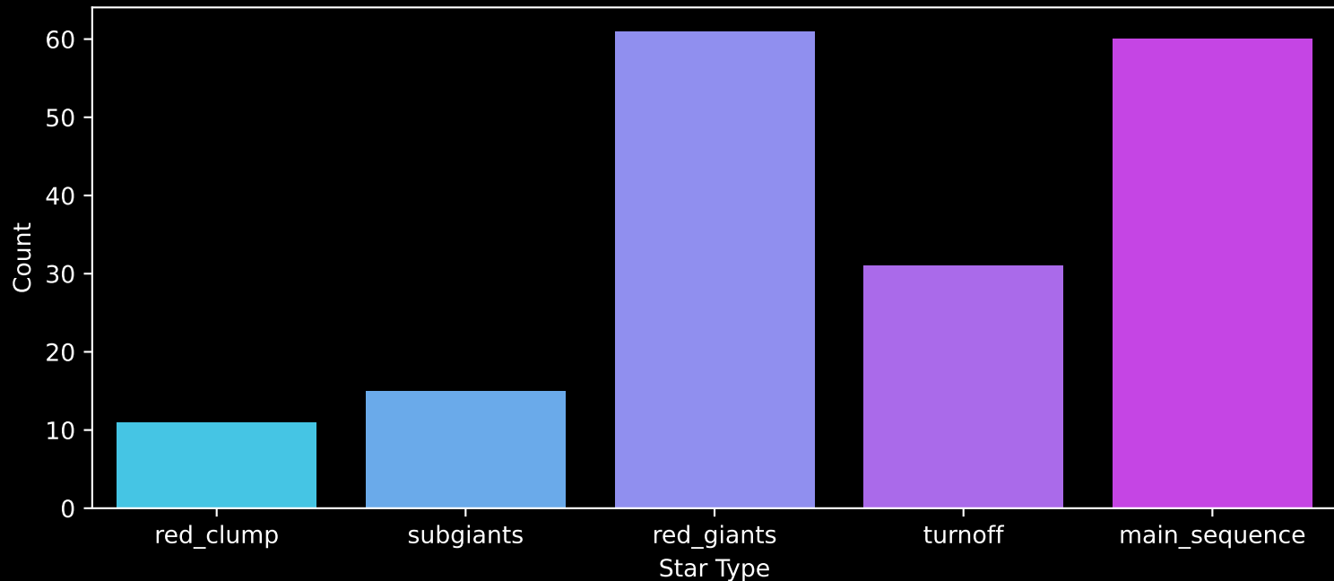
APOGEE DR17 Field: [CVZTILE_103+33_btx] Count plot of Star Type
