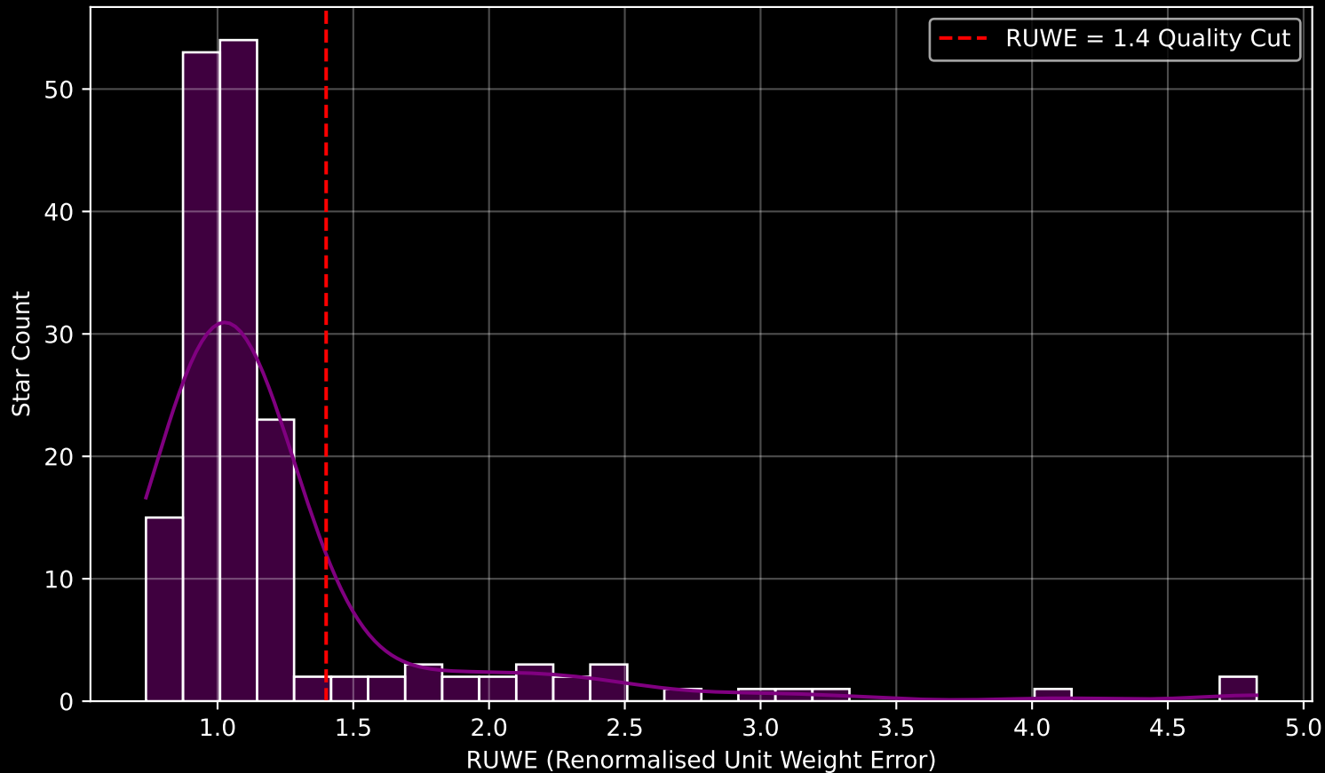
GAPOGEE DR17 Field [CVZTILE_103+33_btx] RUWE Distribution (n= 173)
