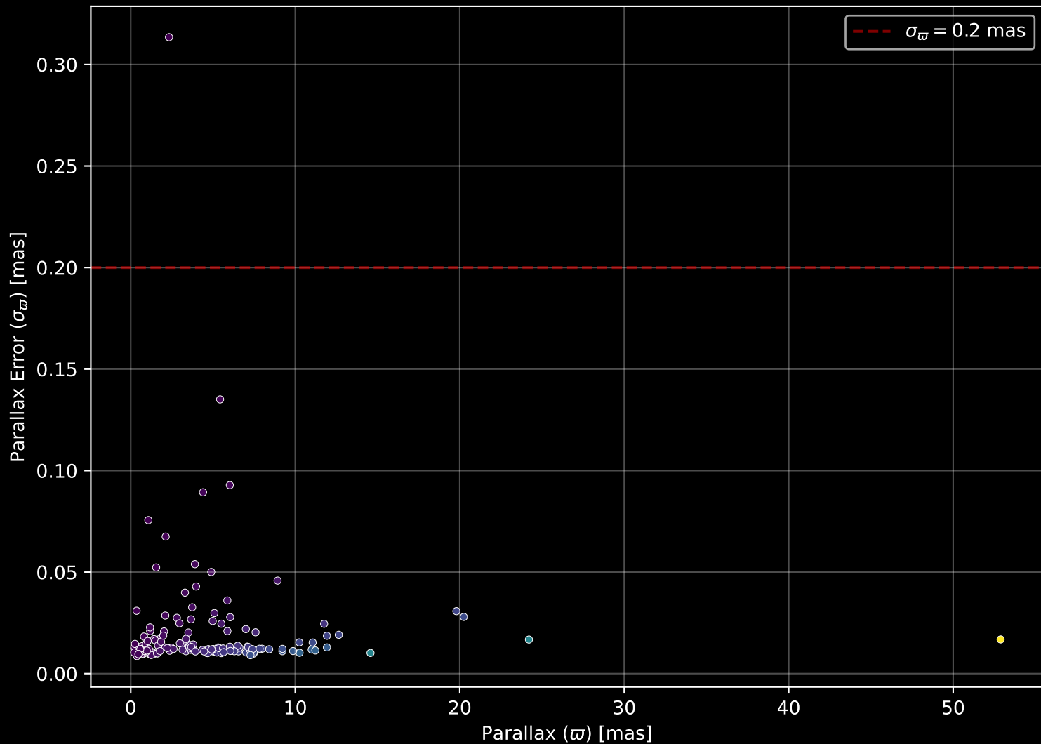
APOGEE DR17 Field: [CVZTILE_103+33_btx] Parallax Quality (n= 178)
