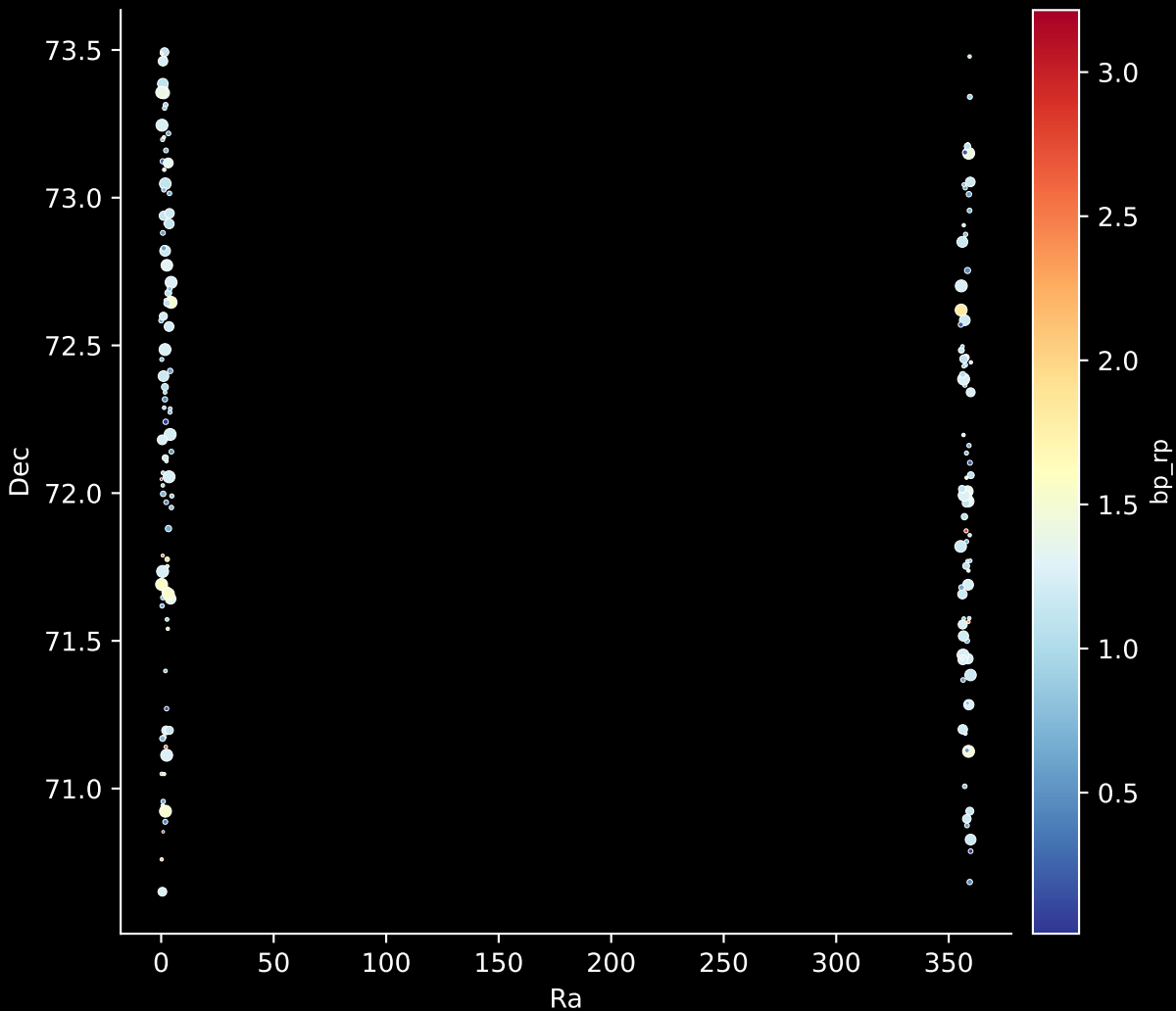
APOGEE DR17 Field: [CVZTILE_103+33_btx] Stars: 178
