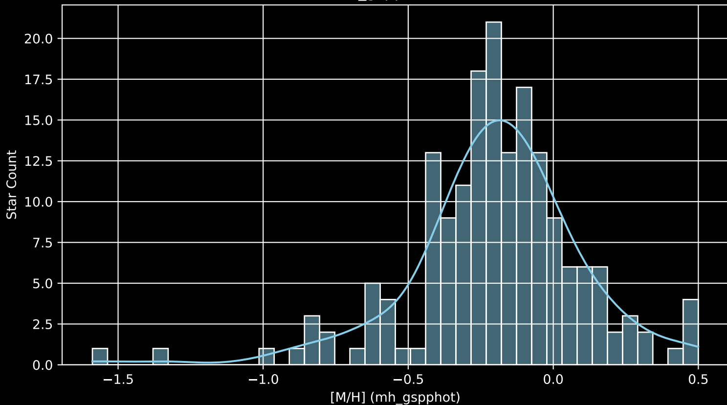
APOGEE DR17 Field: [CVZTILE_103+33_btx [M/H] (mh_gspphot) (n= 175)
