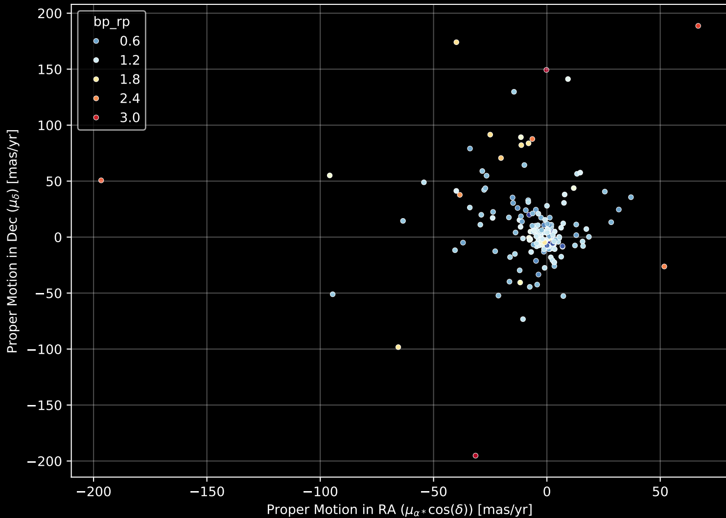
APOGEE DR17 Field: [CVZTILE_103+33_btx] Proper Motion Diagram (n= 178)
